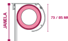
ENROLAMENTO EXTERIOR
